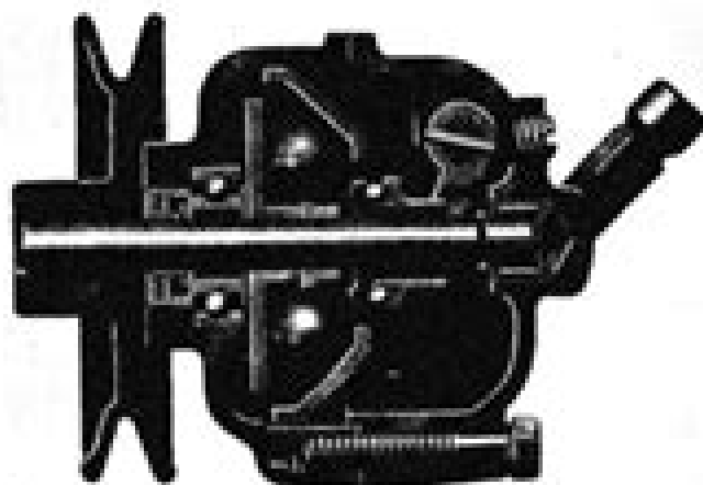
FIG. 13—GOVERNOR
