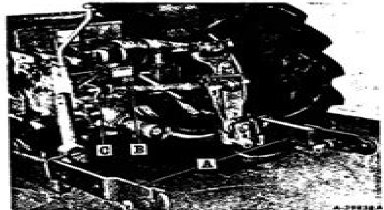
Illustr. 92A Three-point adapter including coupling beams (A), adjustable depth control link (B), and fixed pivot bracket (C).
