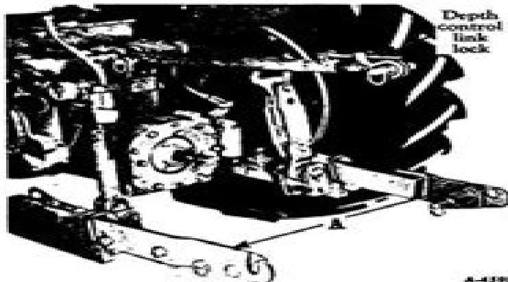
Illustr. 92 Three-point adapter consisting of two coupling beams (A) only. Adjustable link (B) is required but is separately furnished to avoid duplication.
