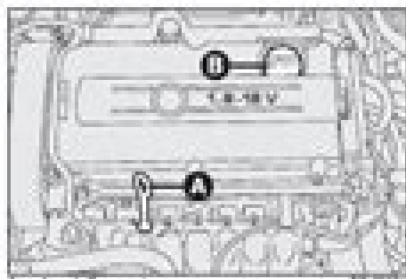
fig. 6 - 1.8 versions
