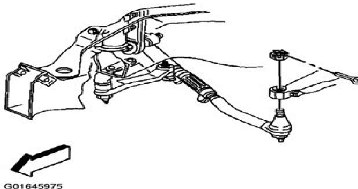
Fig. 8: Installing Castellated Nut Courtesy of GENERAL MOTORS CORP.
