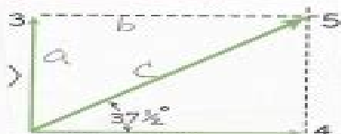
Figure 3.4 ▲ The 3-unit and 4-unit vectors add to produce a resultant vector of 5 units, at 37.5° from the horizontal.
