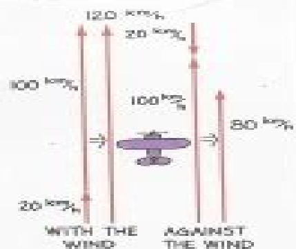
Figure 3.2 ▲ The airplane's velocity relative to the ground depends on the airplane's velocity relative to the air and on the wind's velocity.
