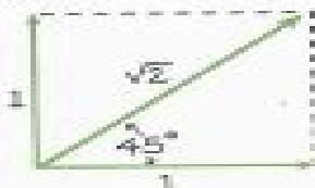
Figure 3.5 ▲ The diagonal of a square is \sqrt{2} , or 1.414, times the length of one of its sides.
