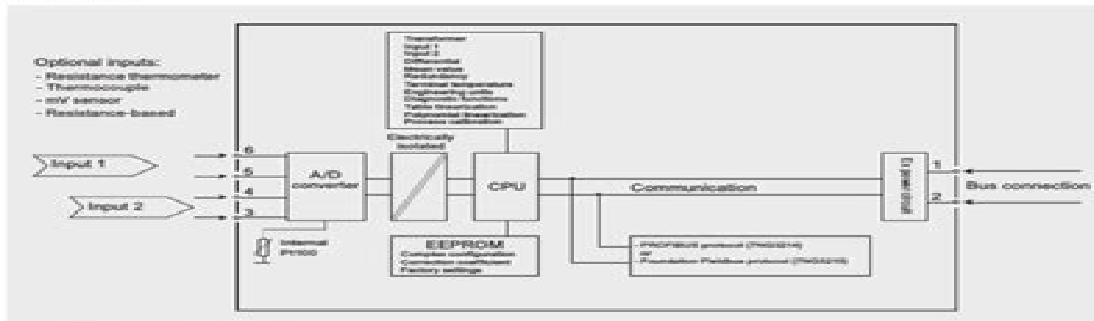
SITRANS TH400, function diagram
