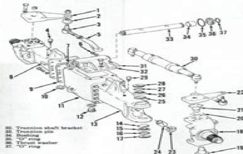
Fig. 5—Exploded view of David Brown front drive axle used on some models showing component parts and their relative positions.
