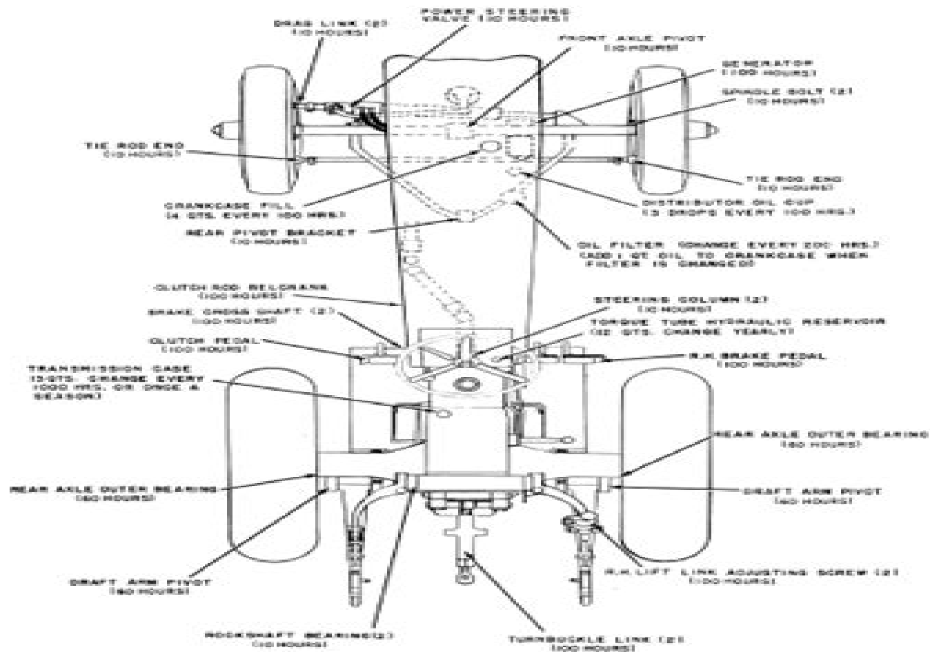
Fig. 8. "540" and "540C" Utility Tractor
