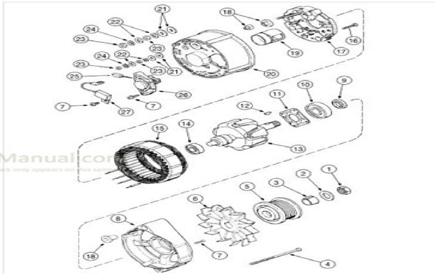
95 Ampere Alternator
