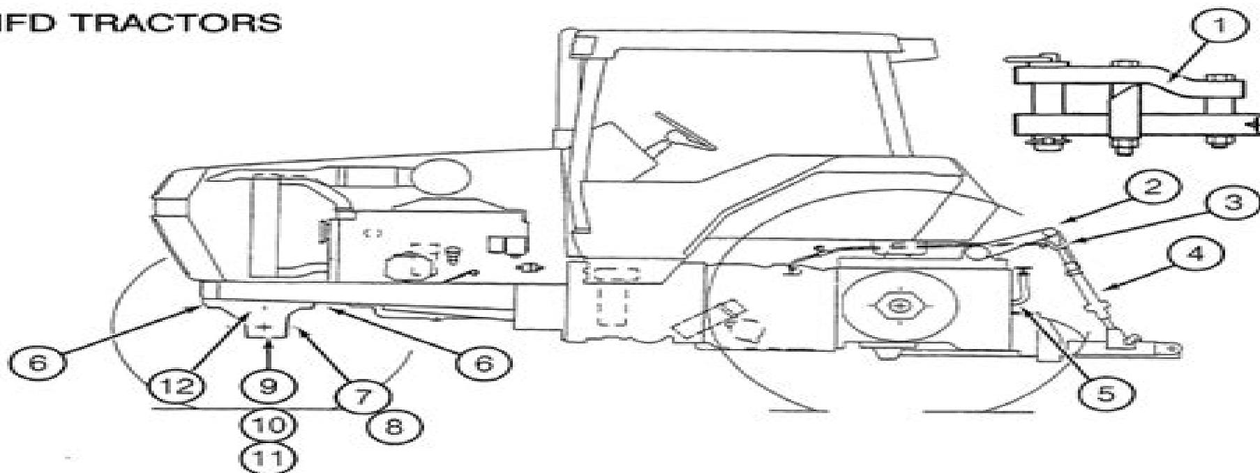
Lift Link Pin - (1 each side) and Upper RH Lift Cylinder Pin
