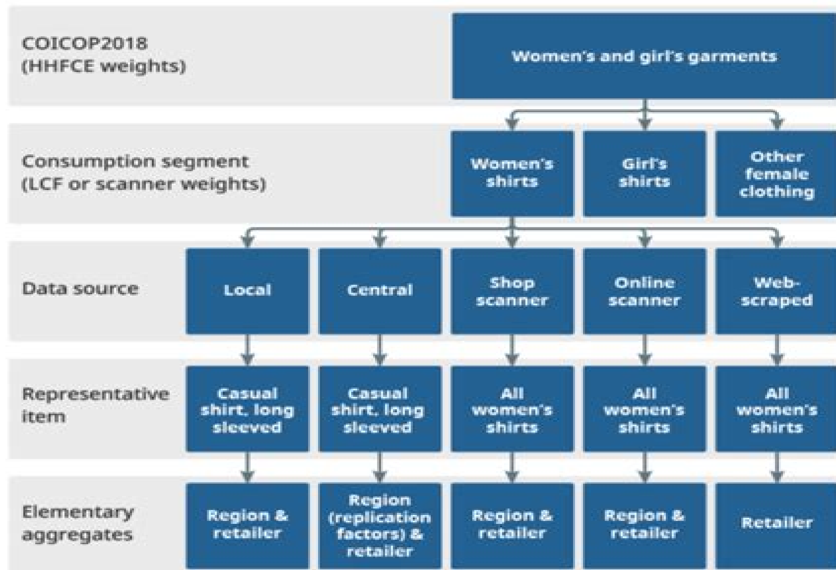
Figure 1: Proposed future aggregation structure for CPIH and CPI below the lowest level of the COICOP hierarchy
