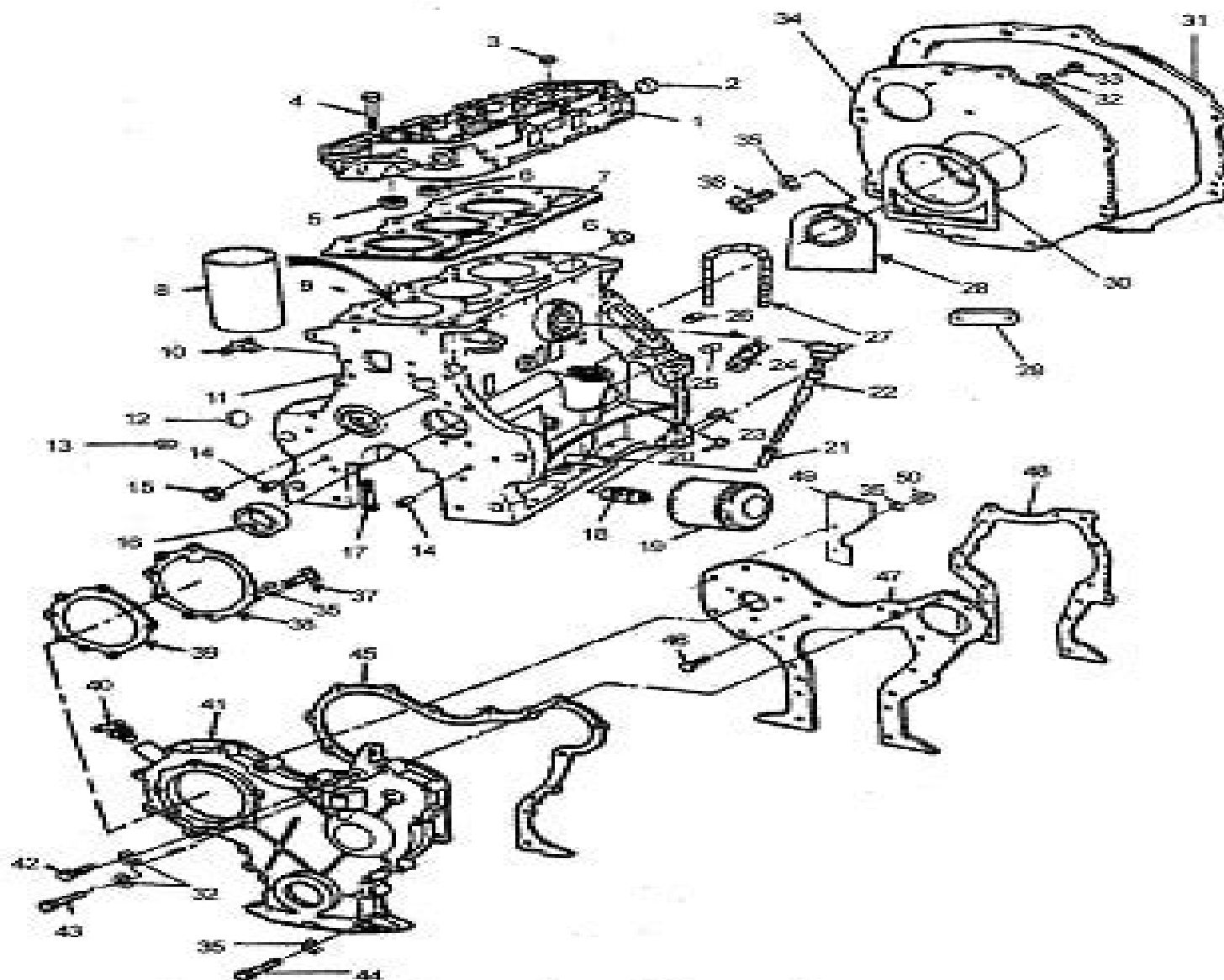
CYLINDER BLOCK & CYLINDER HEAD
