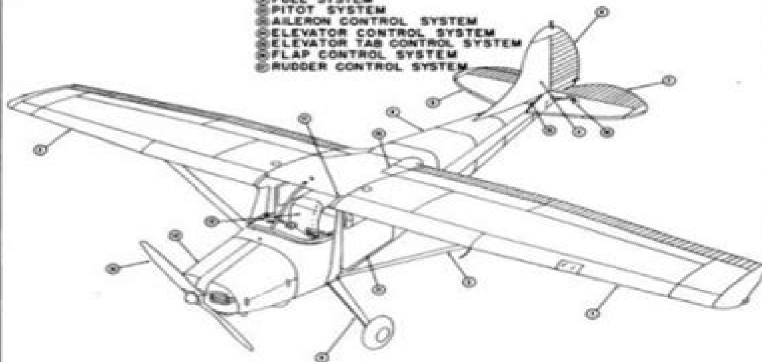
FIGURE 1— AIRPLANE ASSEMBLY
