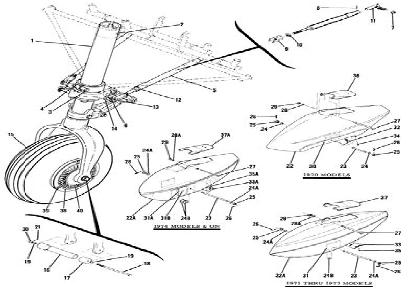
Figure 32. Nose Gear Installation
