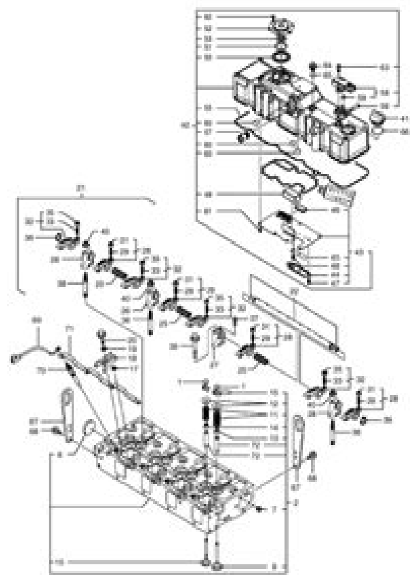
Fig. 014 CYLINDER HEAD & BONNET
