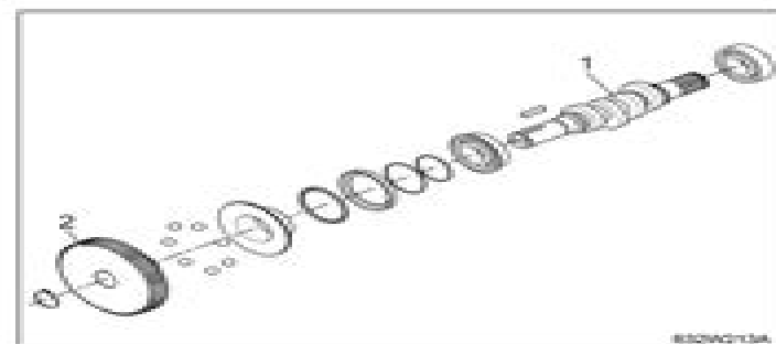
(1) Fuel Camshaft (2) Injection Pump Gear
