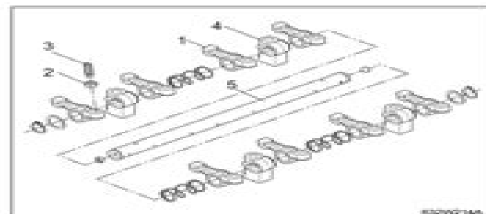
(1) Rocker Arm (4) Rocker Arm Bracket (2) Lock Nut (5) Rocker Arm Shaft (3) Adjusting Screw
