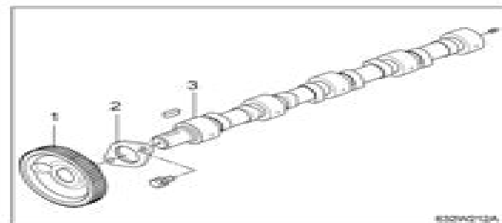
(1) Cam Gear (3) Camshaft (2) Camshaft Stopper
