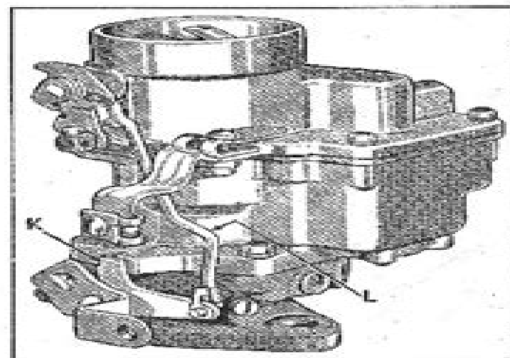
Figure 5 Fast Idle Adjustment
