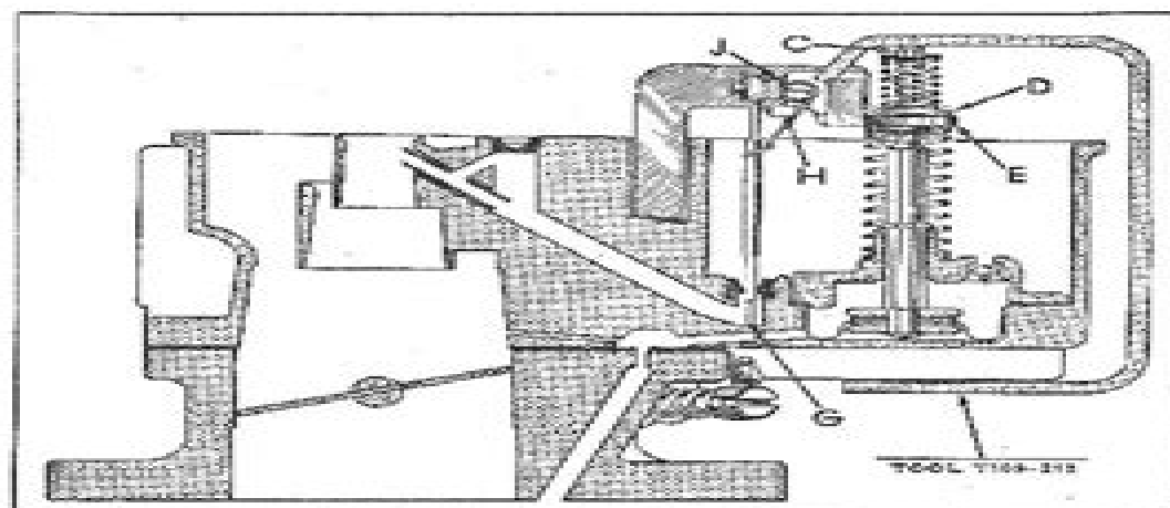
Figure 4 Metering Rod Adjustment
