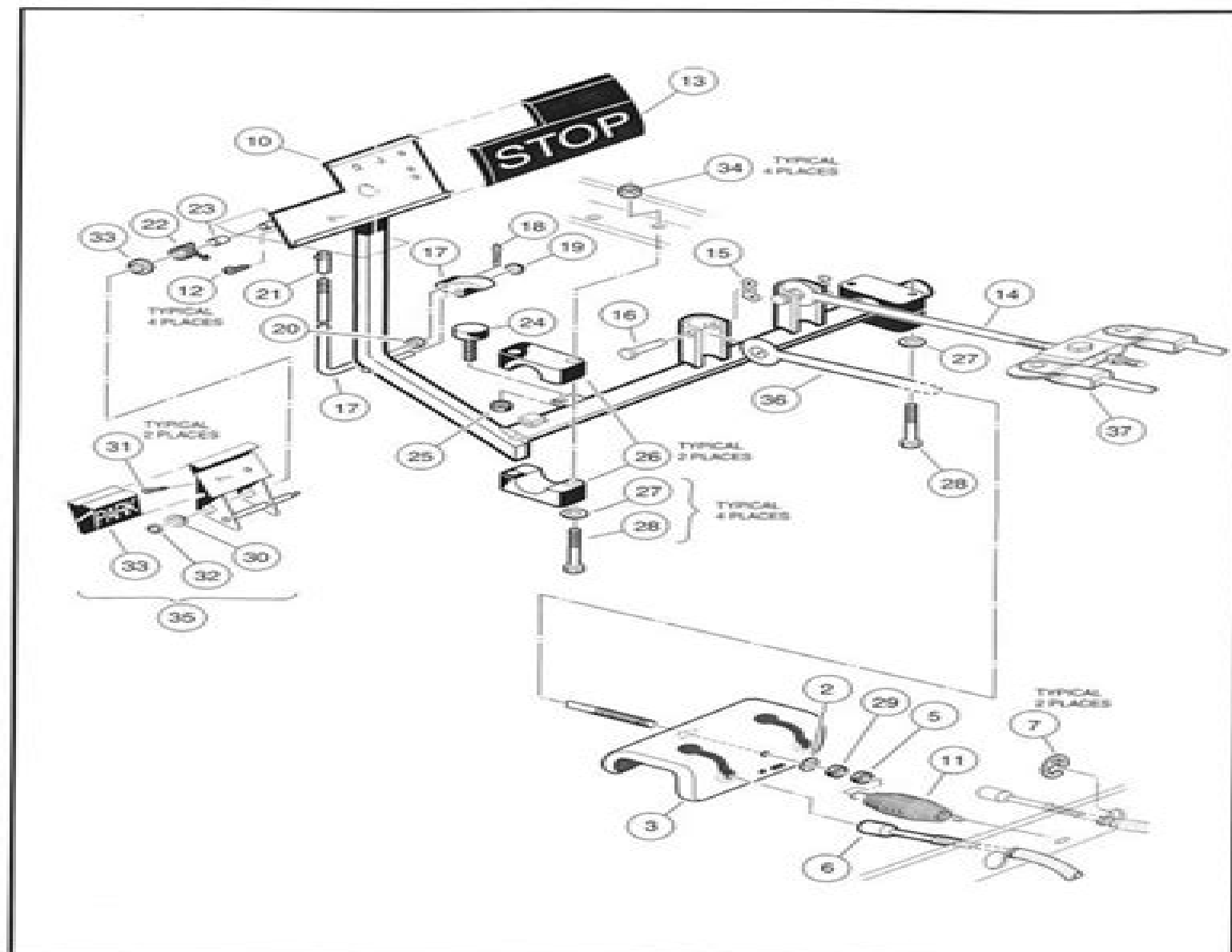
Figure 5-2 Brake and Park Brake Pedal Assembly and Mounting – Four-Wheel Brake Vehicles
