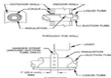
Fig. 1 - Connecting Tubing Installation
