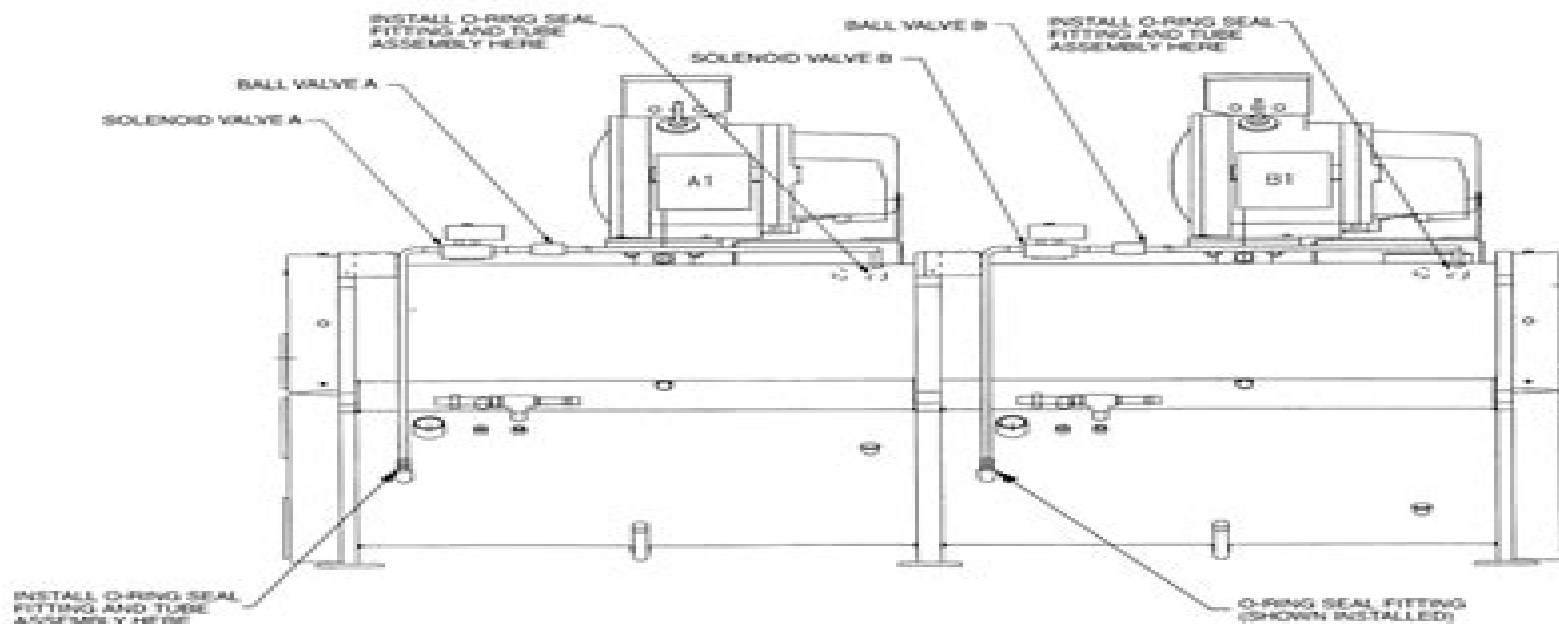
Fig. 2 — Installing Fittings and Valves, 30HX (Typical)
