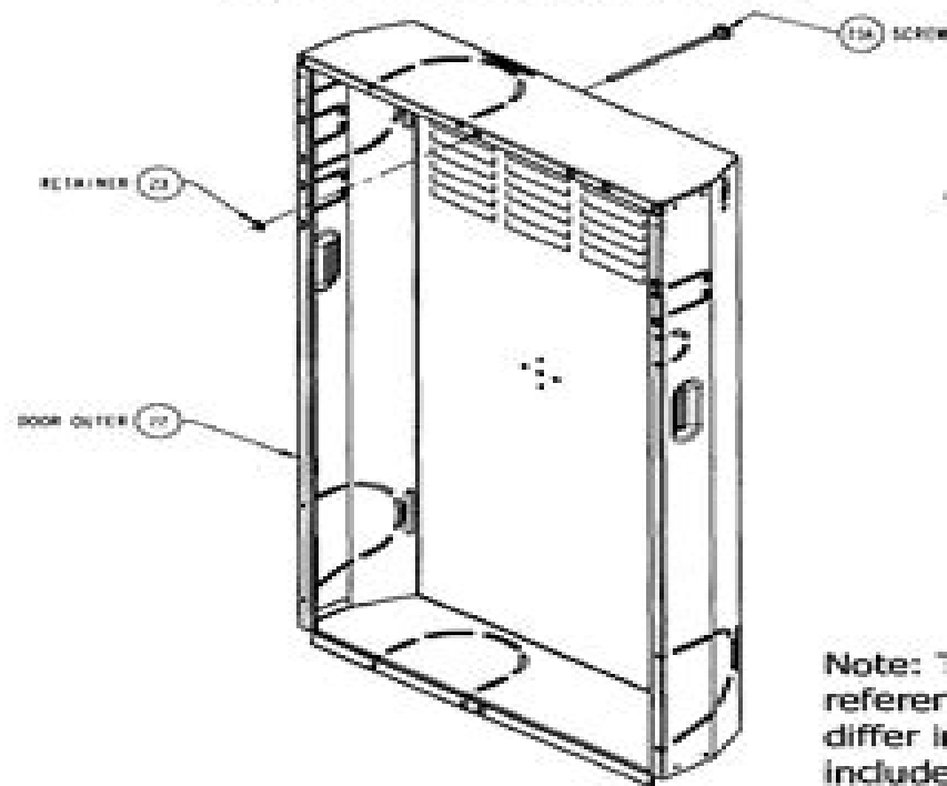
Outer Door Assy (21)
