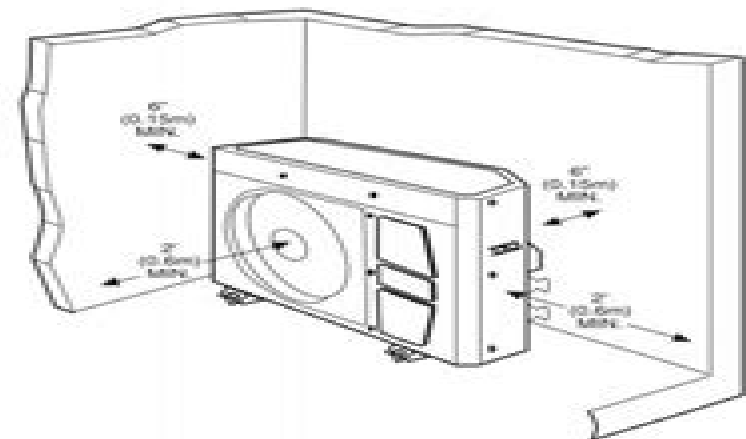
Fig. 1 — 38BNB,BNE Outdoor Unit Clearances
