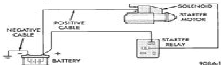
Fig. 1 Starting System Components
