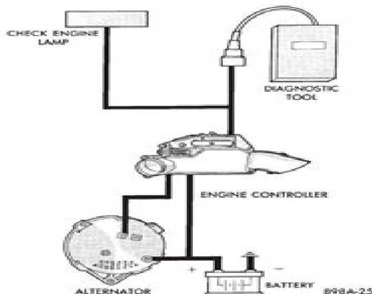
Fig. 2 Charging System Components
