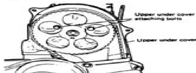
Installing upper under cover (4G33)
