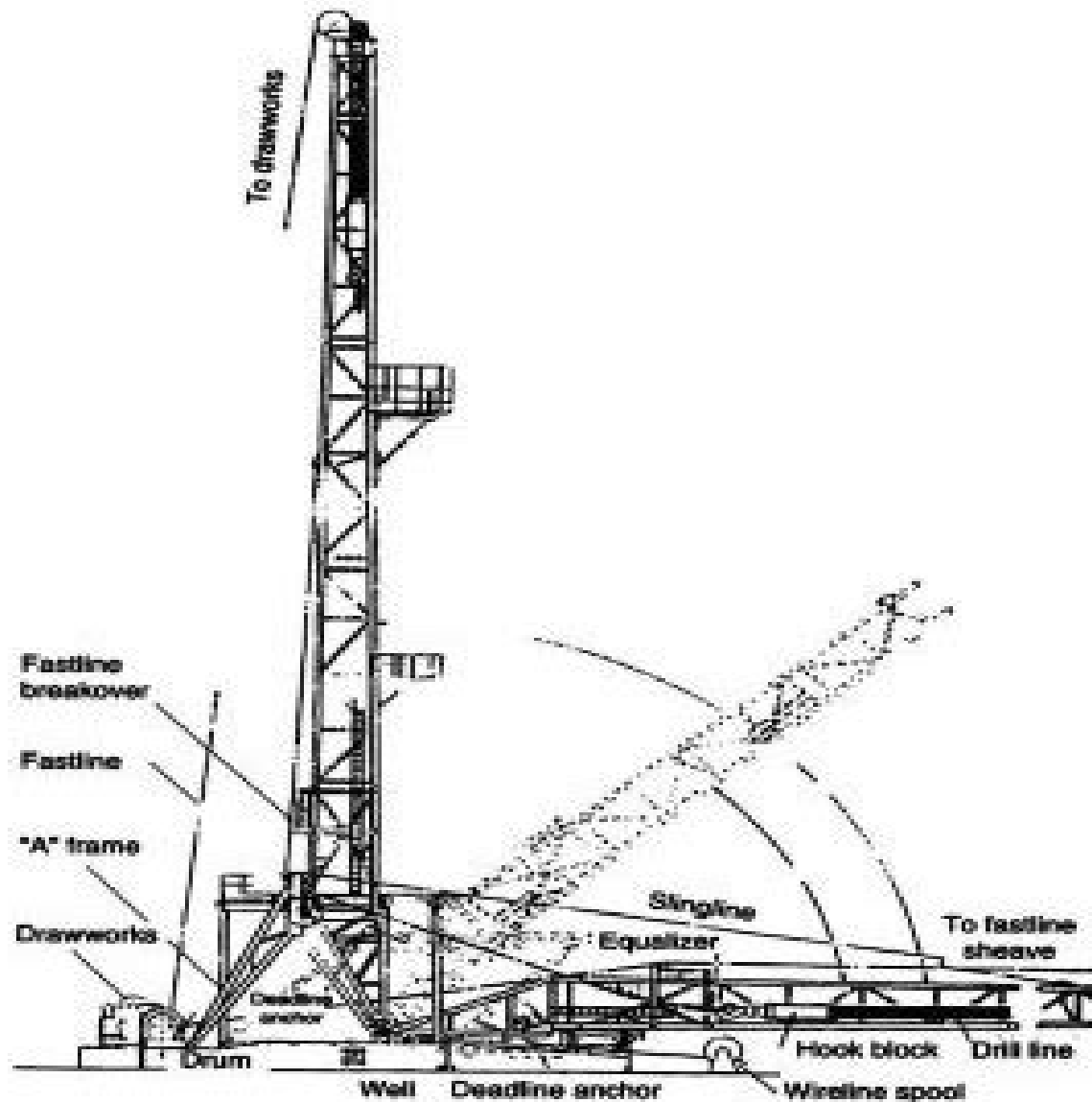
Schematic diagram showing how a mast is erected (Source: Branham Industries Inc.).
