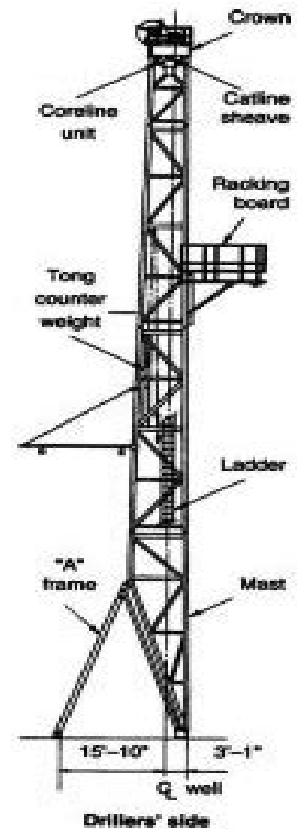
Drilling rig mast (Source: Branham Industries Inc.).
