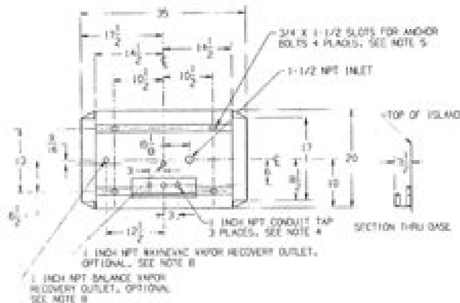
BASE DIMENSIONS
