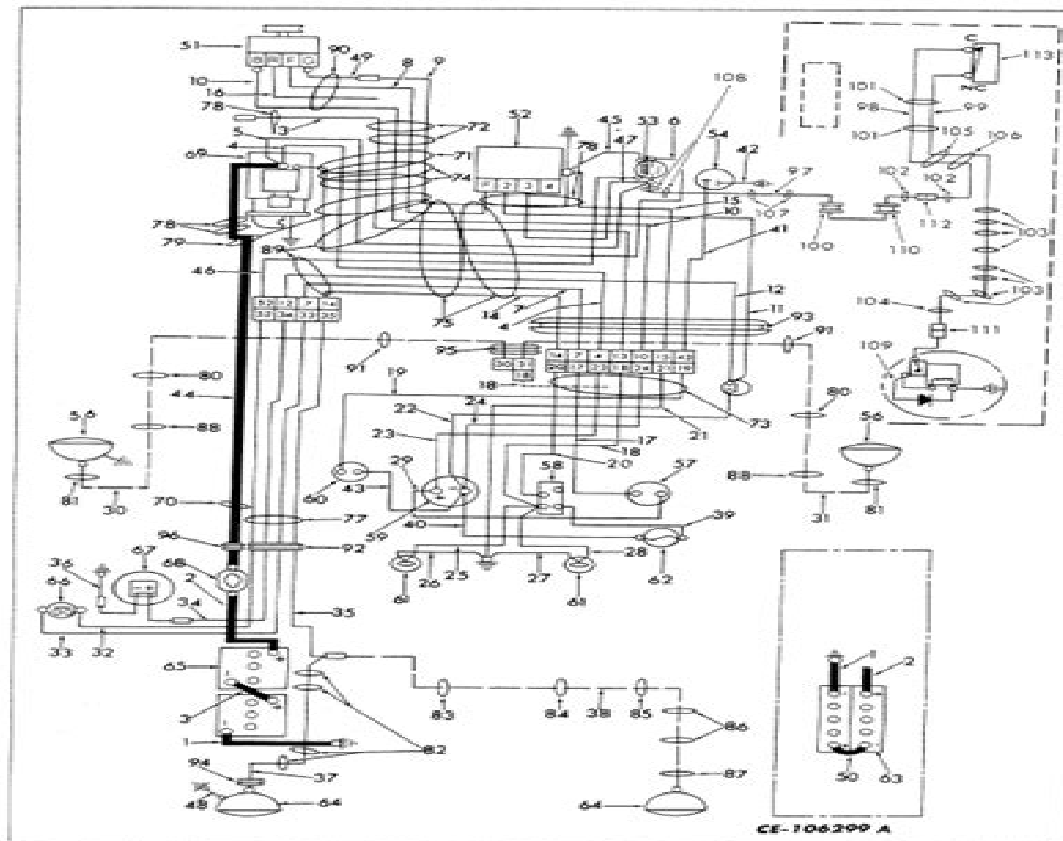
Illustr. 8 Wiring Diagram (Model 100 and 125 Series E)
