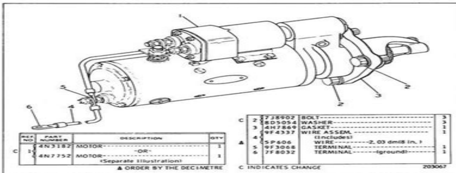
7S3622 STARTING MOTOR GROUP—24 Volt—Type 4 Part of 7S9854 & 1P271 Starting Arrangements listed on Pages 120D & 121 4N3182 & 4N7752 Motor parts are shown on Pages 121B, 121C, 121D, 121G & 121H
