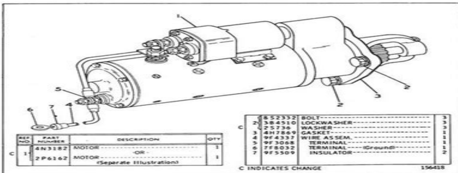
7S3622 STARTING MOTOR GROUP—24 Volt—Type 3 Part of 7S9854 & 1P271 Starting Arrangements listed on Pages 120D & 121 4N3182 & 2P6162 Motor parts are shown on Pages 121B through 121F
