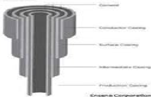
Typical Well Casing Diagram
