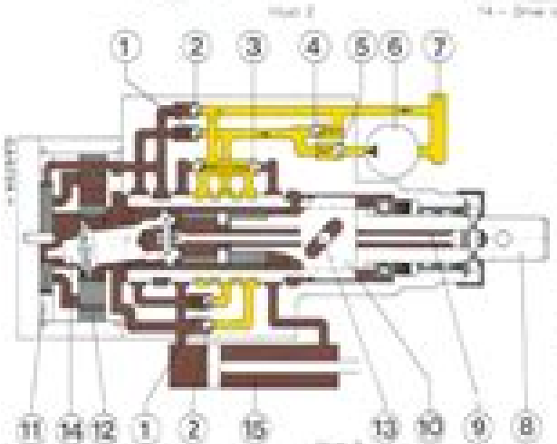
Sectional position, piston rod seal recirculation valve
