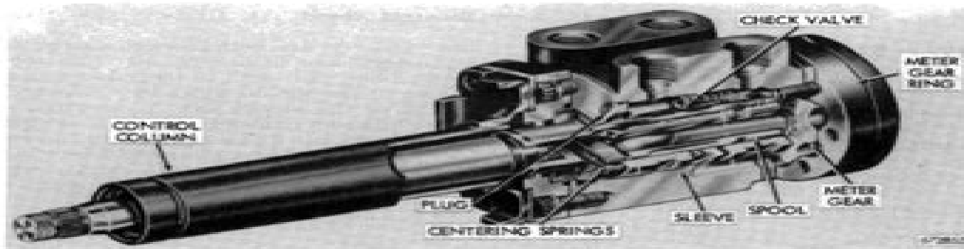
Figure 1 - Typical Steering Valve
