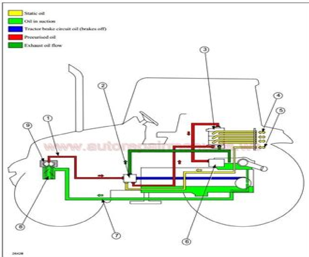
Diagram of the hydraulic trailer brake circuit
