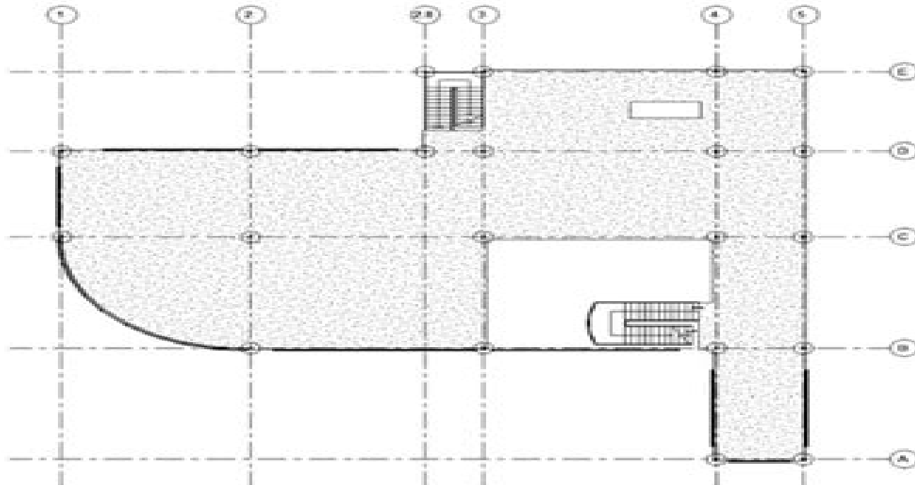
FIGURE 7-3.8 Level 2 – Structural Framing Plan, columns added.
