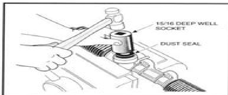
Figure 7-13 Press In Dust Seal
