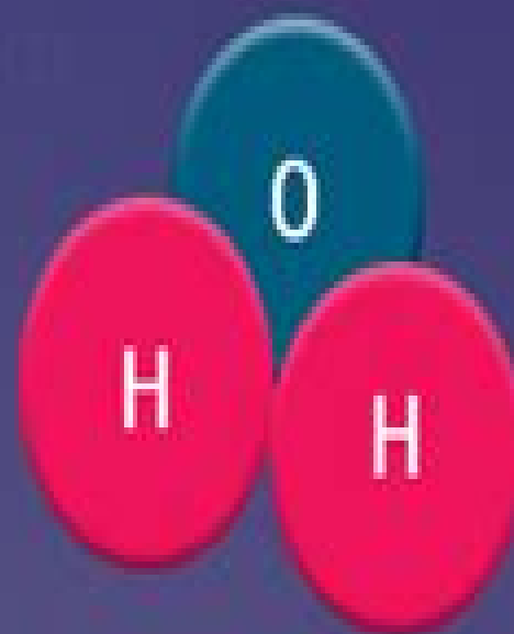
Water ( H2O )
