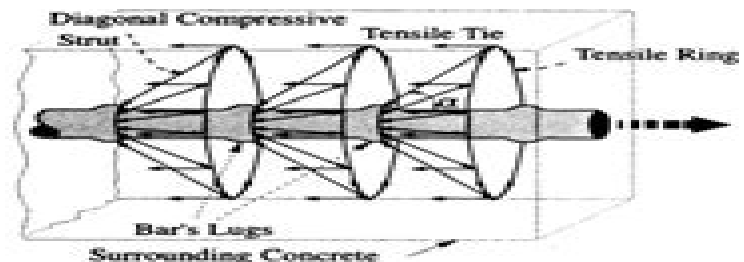
Fig. 1 Tensile ring force caused by diagonal bond struts
