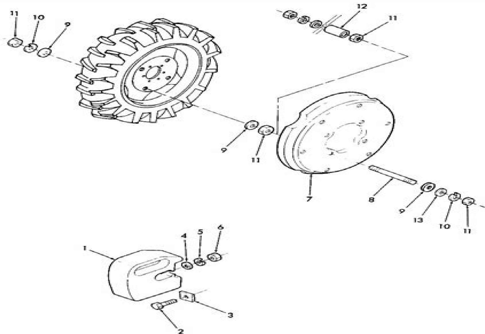
FIG. 1B1 — FRONT END & REAR WHEEL WEIGHT
