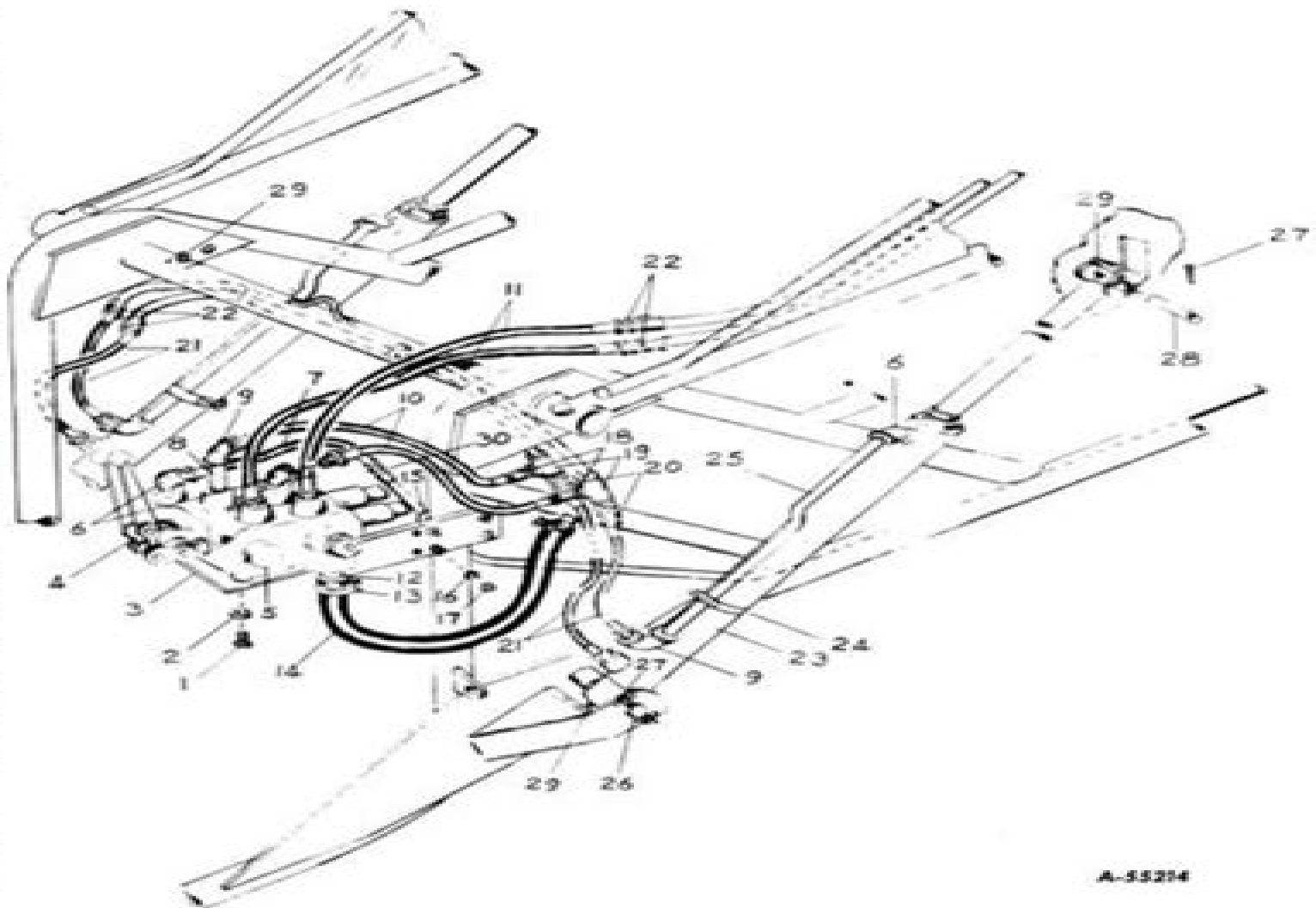
FIGURE 6, CONTROL VALVE AND LIFT CYLINDER CONNECTIONS
