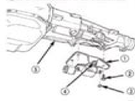
Fig. 36 Engine Rear Mount—4x4 Automatic Transmission 1 - ENGINE REAR MOUNT 2 - BOLT 3 - NUT 4 - THROUGH-BOLT NUT 5 - TRANSMISSION
