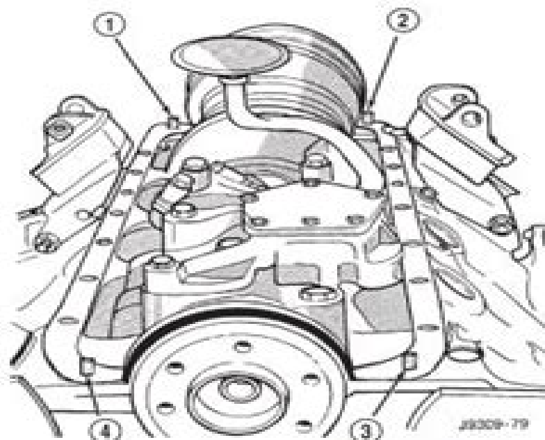
Fig. 54 Position of Dowels in Cylinder Block
