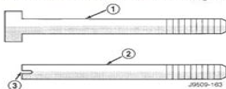
Fig. 53 Fabrication of Alignment Dowels
