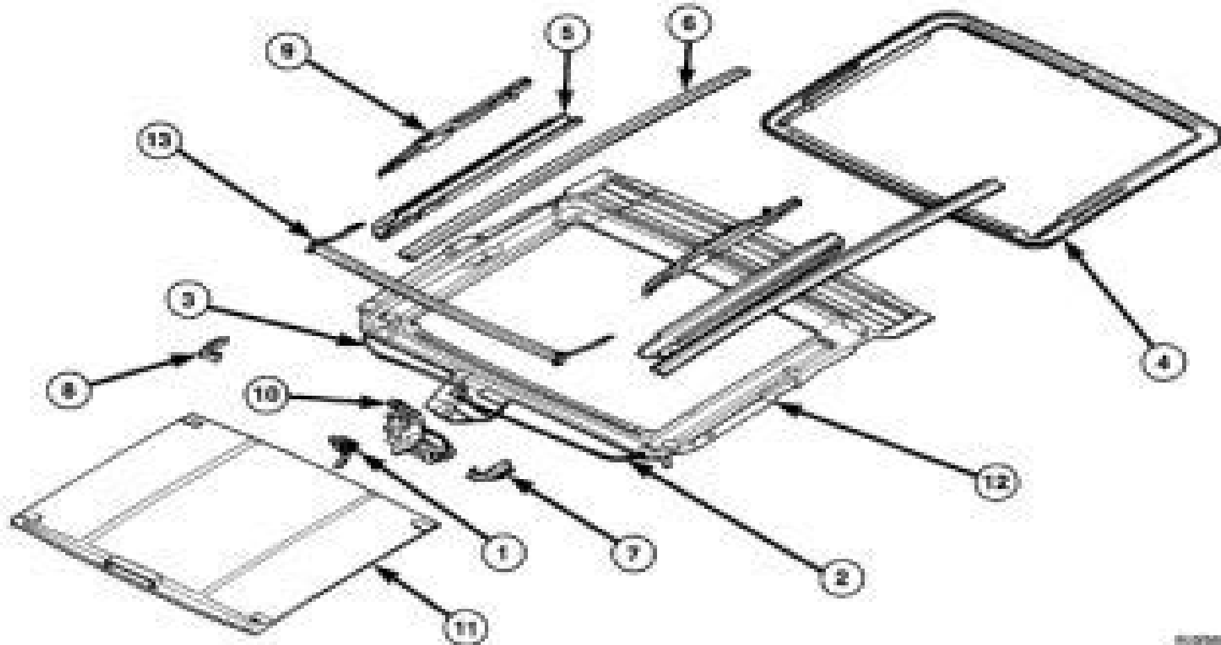
Fig. 1 Sunroof Components
