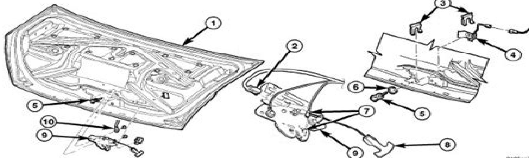
Fig. 3 DECKLID LATCH ASSEMBLY
